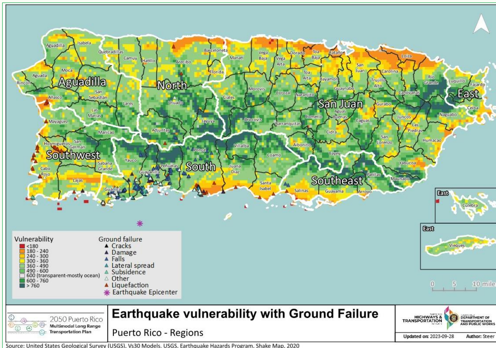
Figure 6.8: Puerto Rico Earthquake Vulnerability According to Vs30 USGS Model and Principal Ground Failure Affections due to 2020 Earthquakes
